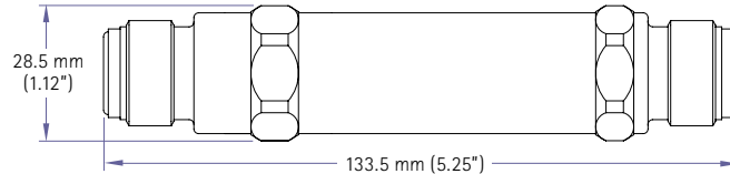
WGMS 32PRU 3/8" Gasket Seal, Male Inlet/outlet
