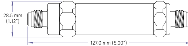
WGMS 32PRU 3/8" Gasket Seal, Male Inlet/outlet
